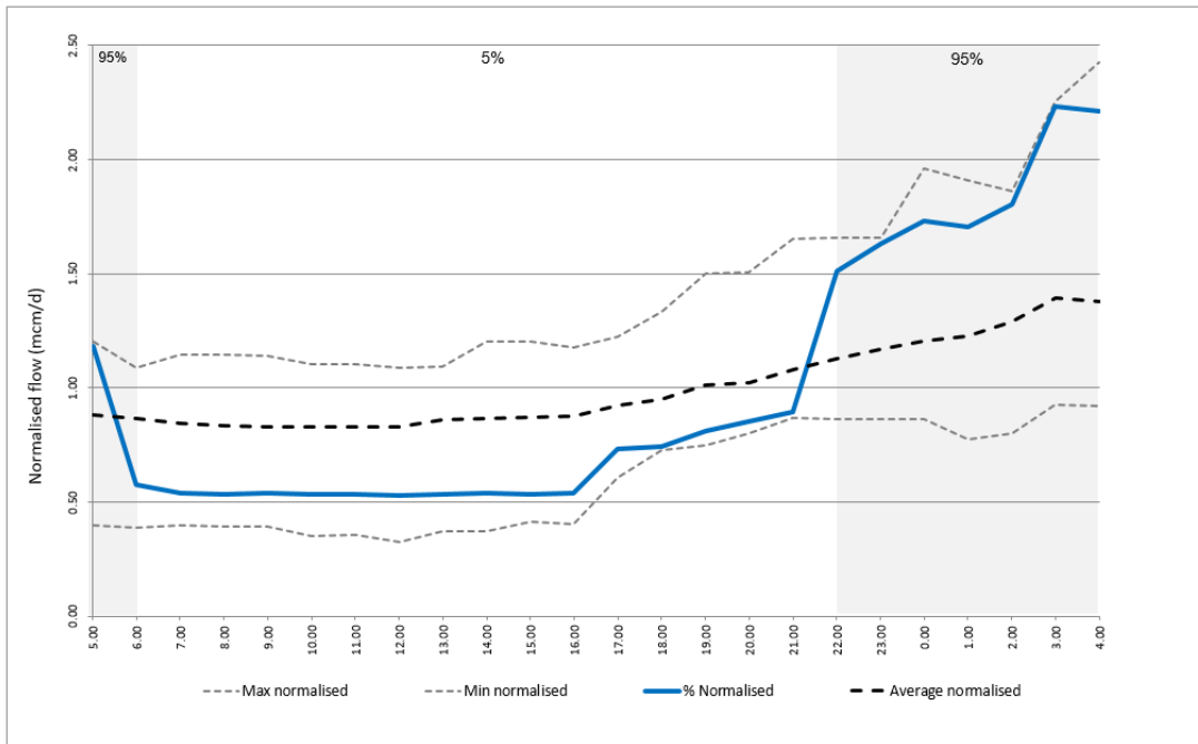
Figure 9 Example of a normalised supply profile for a site between 2020 and 2023, with maximum, minimum, and average profiles.
